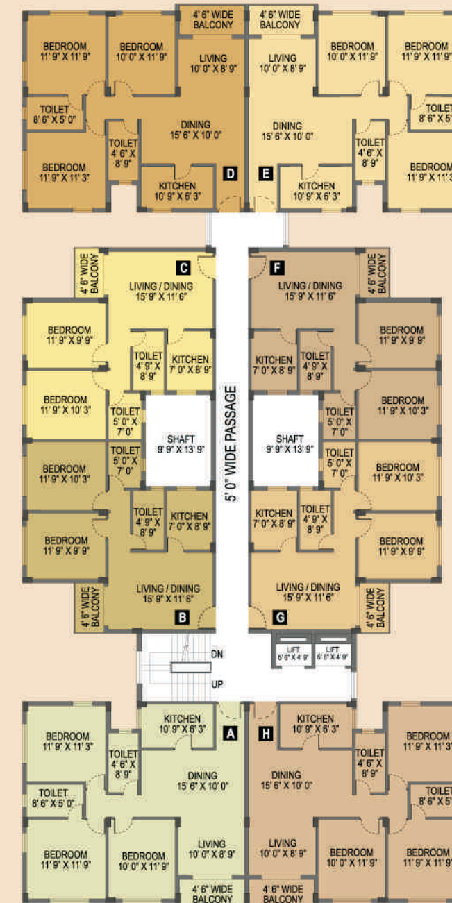
Typical Floor Plan (Block 1)
